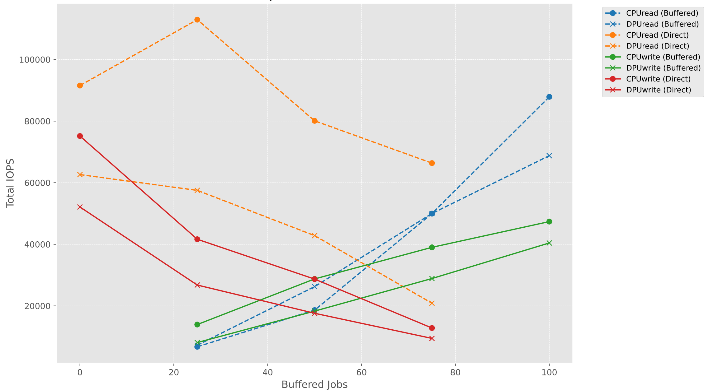
IOPS vs Buffered Jobs (mixed) - SEQ (CPU vs DPU)
